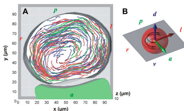
FIGURE 2 Kupffer's vesicle flow extracted from fluorescence data. (A) Particle tracks ( N = 266 ) indicating the fluid streamlines of the steady-state flow within the KV. The three different track colors correspond to the superposition of tracks obtained at different time windows ( 3 \times 15\ \text{s} over a 45\text{-s} period) showing that tracks align over time, indicating a steady state. The particles exhibit a circular motion around the dorso-ventral direction. (B) Schematic display of the spatial orientation (antero-posterior, dorso-ventral, and left-right axis are represented in green, blue, and red, respectively) of the vesicle (red sphere). The black arrows indicate the counterclockwise rotation of the flow (when viewed from the dorsal side). d , dorsal; v , ventral; a , anterior; p , posterior; l , left; and r , right.
